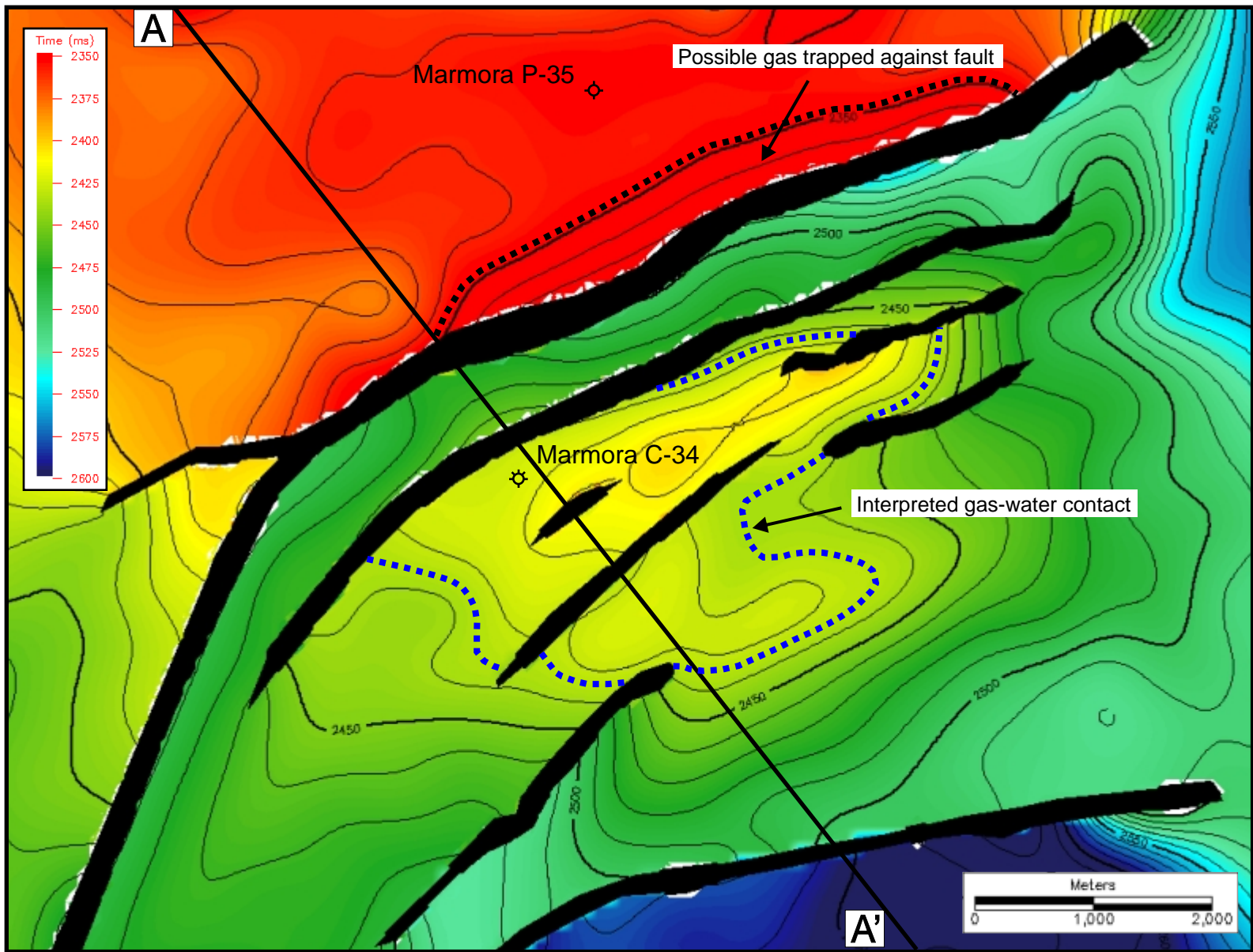
Structure map of the top Missisauga gas sand (Sand 1) encountered in the Marmora C-34 well. The interpreted gas-water contact is noted by the dashed blue line. The location of seismic profile A-A' is also shown.
